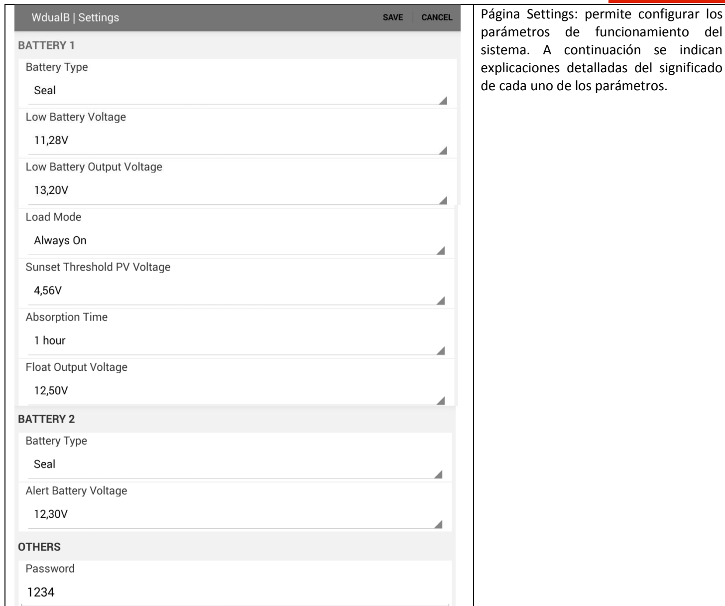
Fig. 4 Bluetooth control
