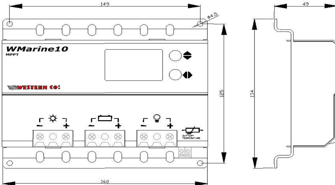
Fig.4 Dimensions
